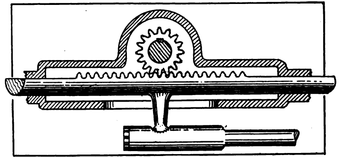
Fig. 35.—Characteristic sketch of rack and pinion.
